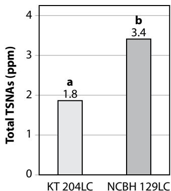
Figure 3. Total TSNA (ppm) for KT 204LC and NCBH 129LC; mean over two years. Bars with different letters are significantly different at the 5% level.
